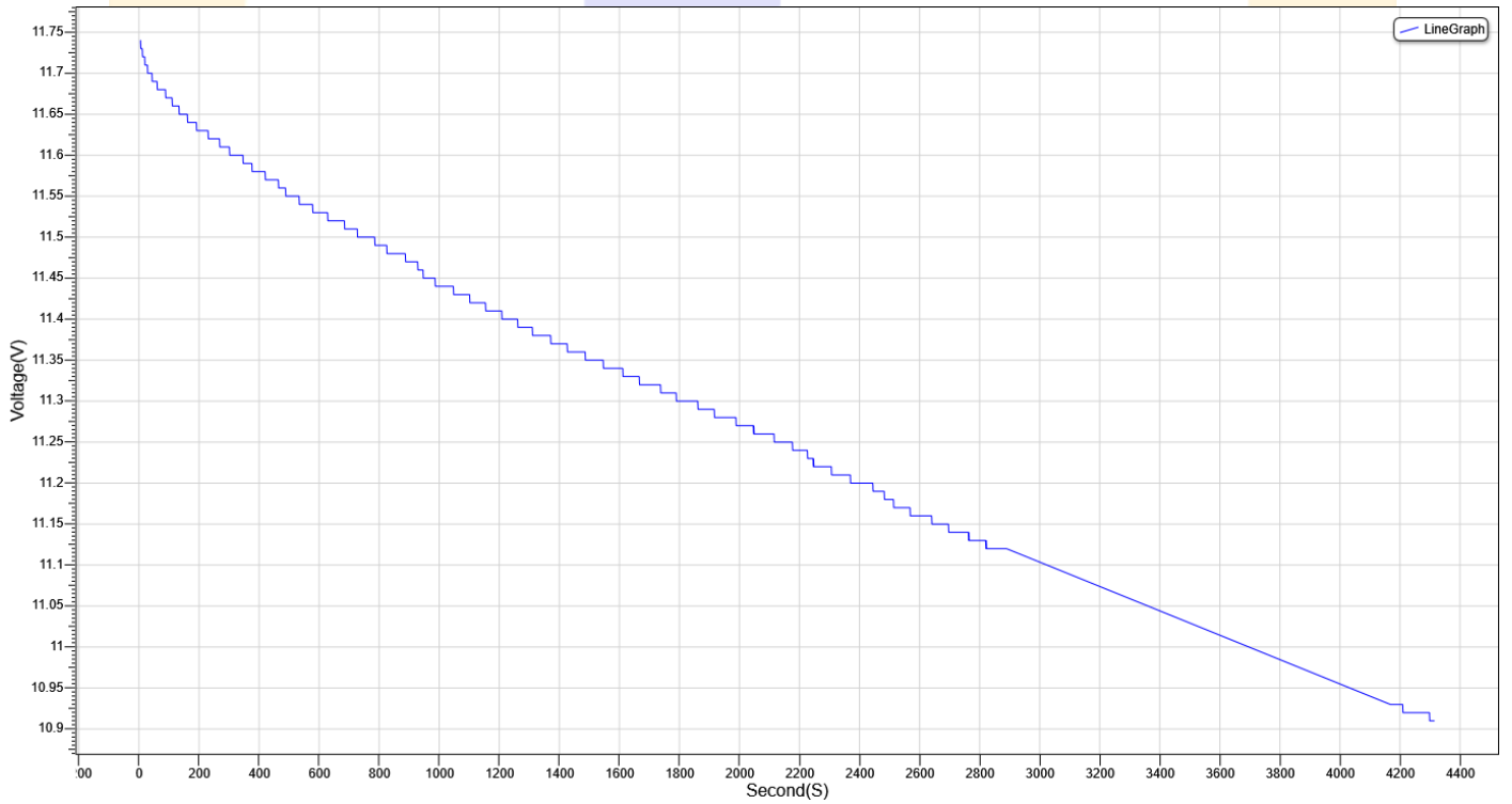
Voltage Versus Time Discharging Graph: -
