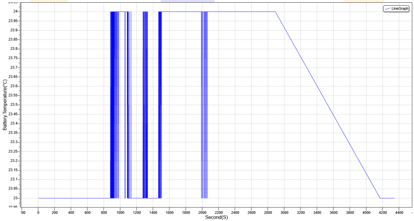
Battery Temperature Versus Time Discharging Graph: -
