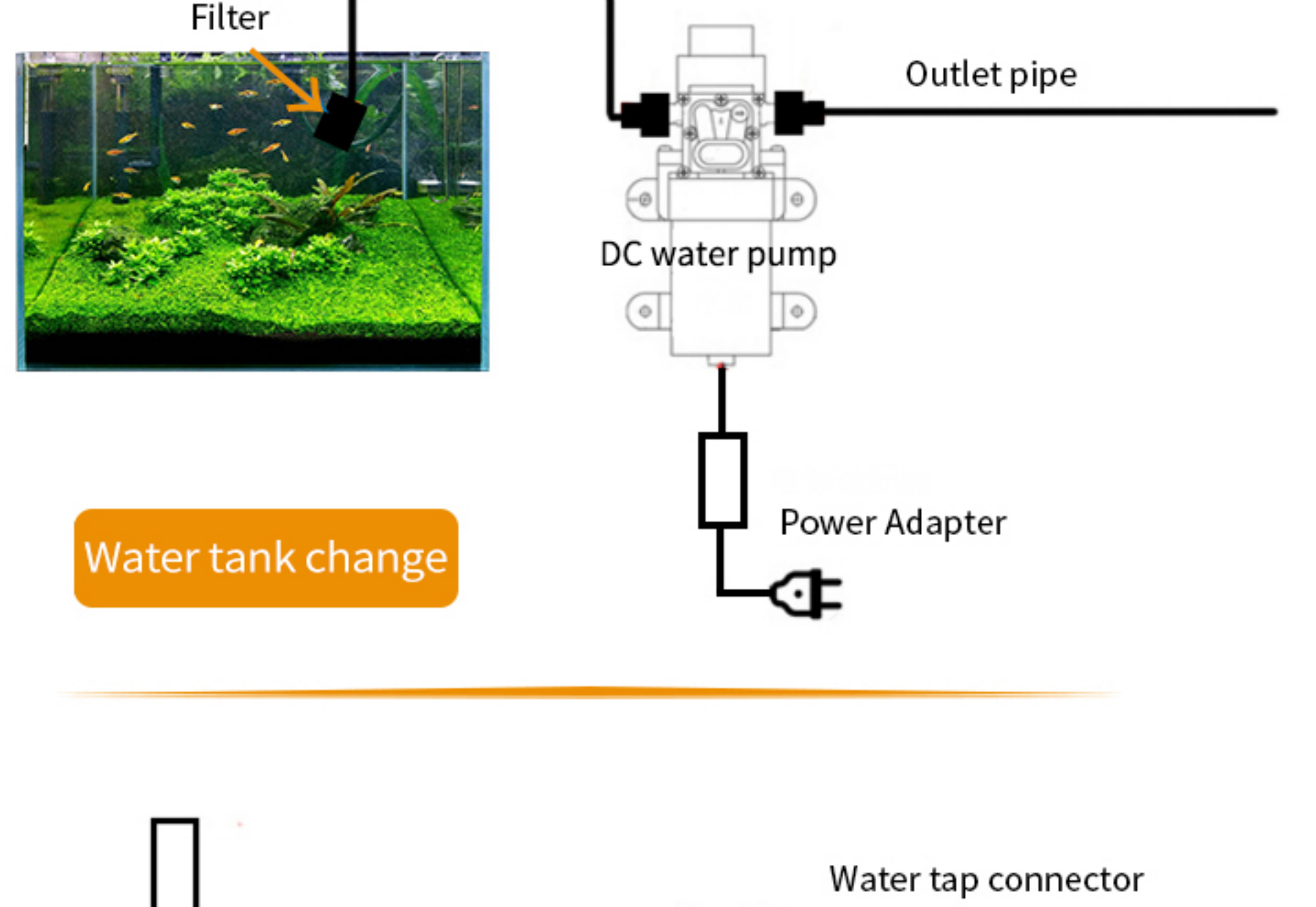
Water Purifier
