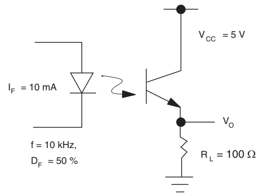
Fig. 10 - Switching Schematic
